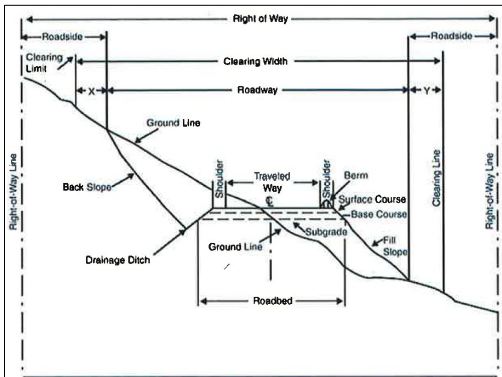
Figure 6.17 Roadway components
